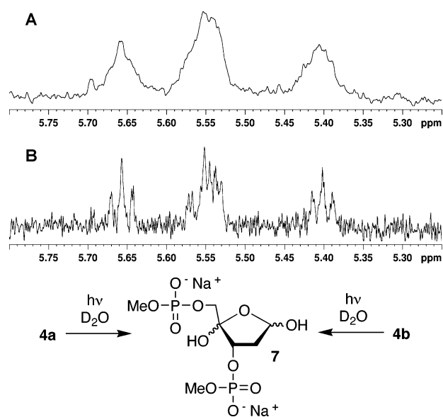
FIGURE 1. ^1\text{H} NMR analysis following photolysis of individual diastereomers of 4 . (A) 4a . (B) 4b .
